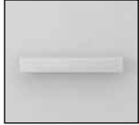
C – Cubic
